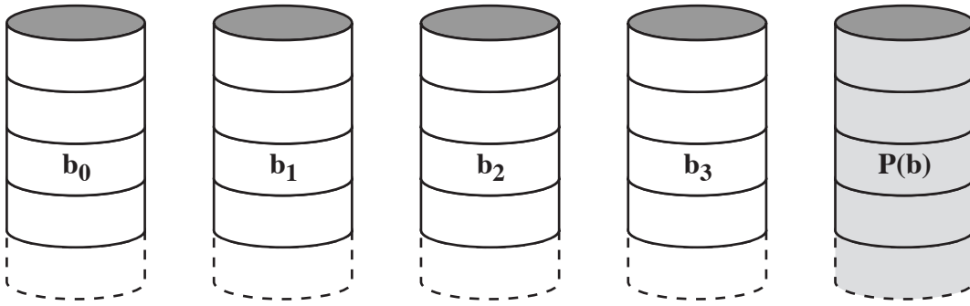
(a) RAID 3 (bit-interleaved parity)
