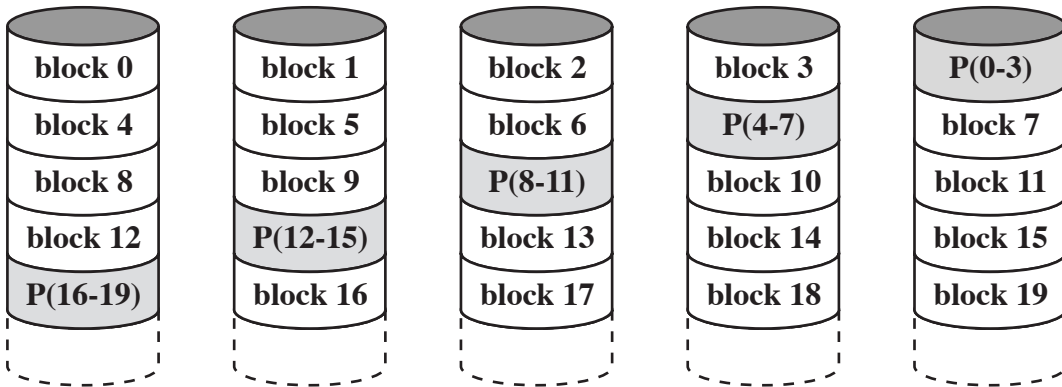
(c) RAID 5 (block-level distributed parity)
