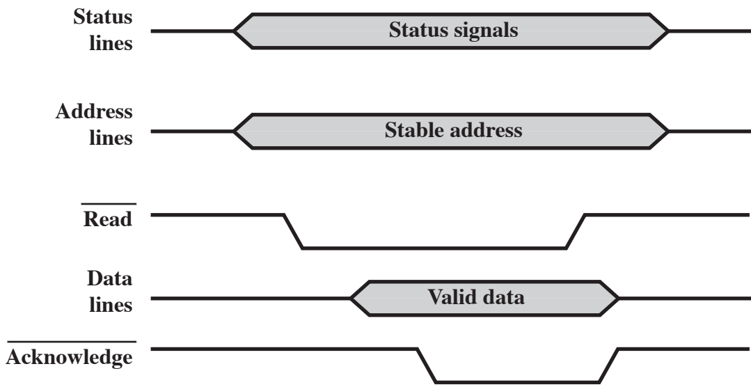
(a) System bus read cycle
