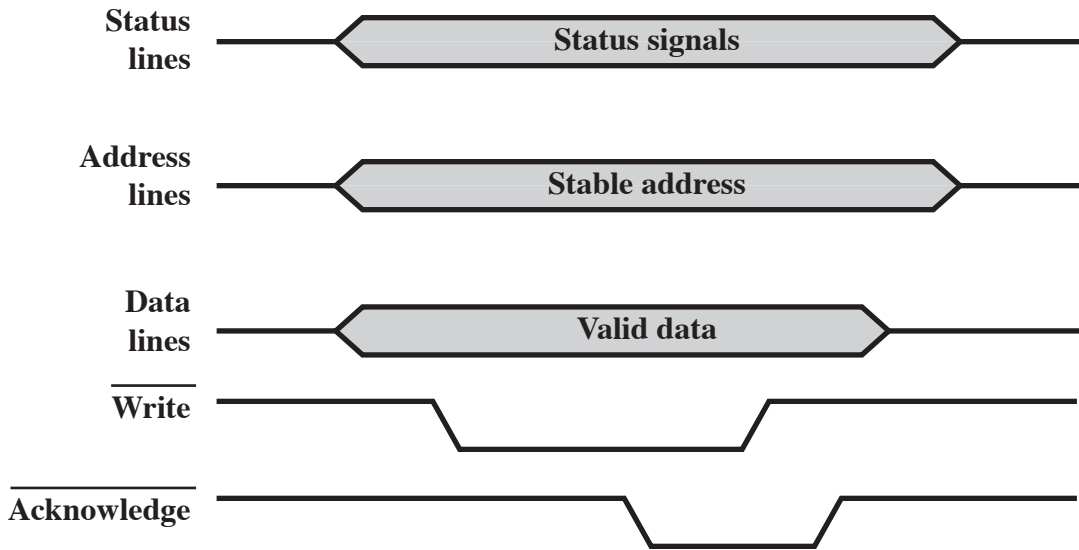
(b) System bus write cycle
