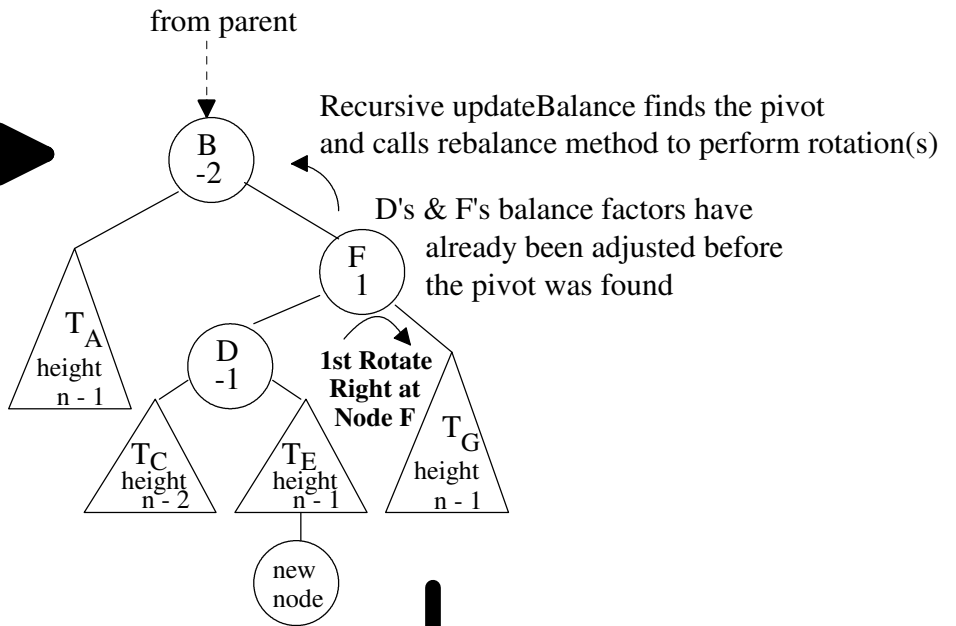
After the addition, but before first rotation:
