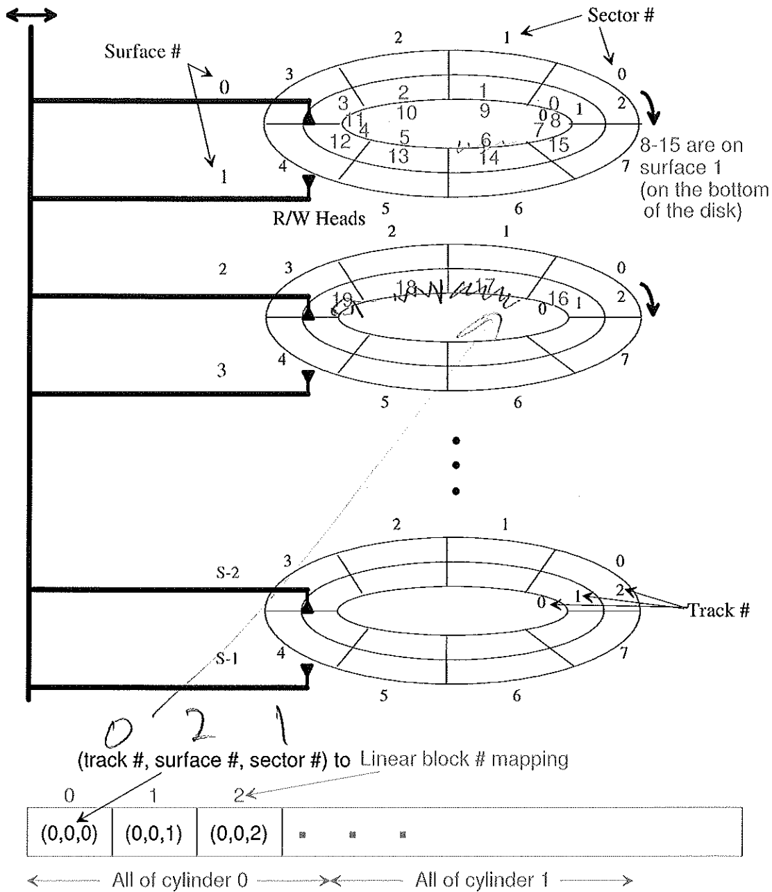
Logical View of Disk as Linear Collection of Blocks
